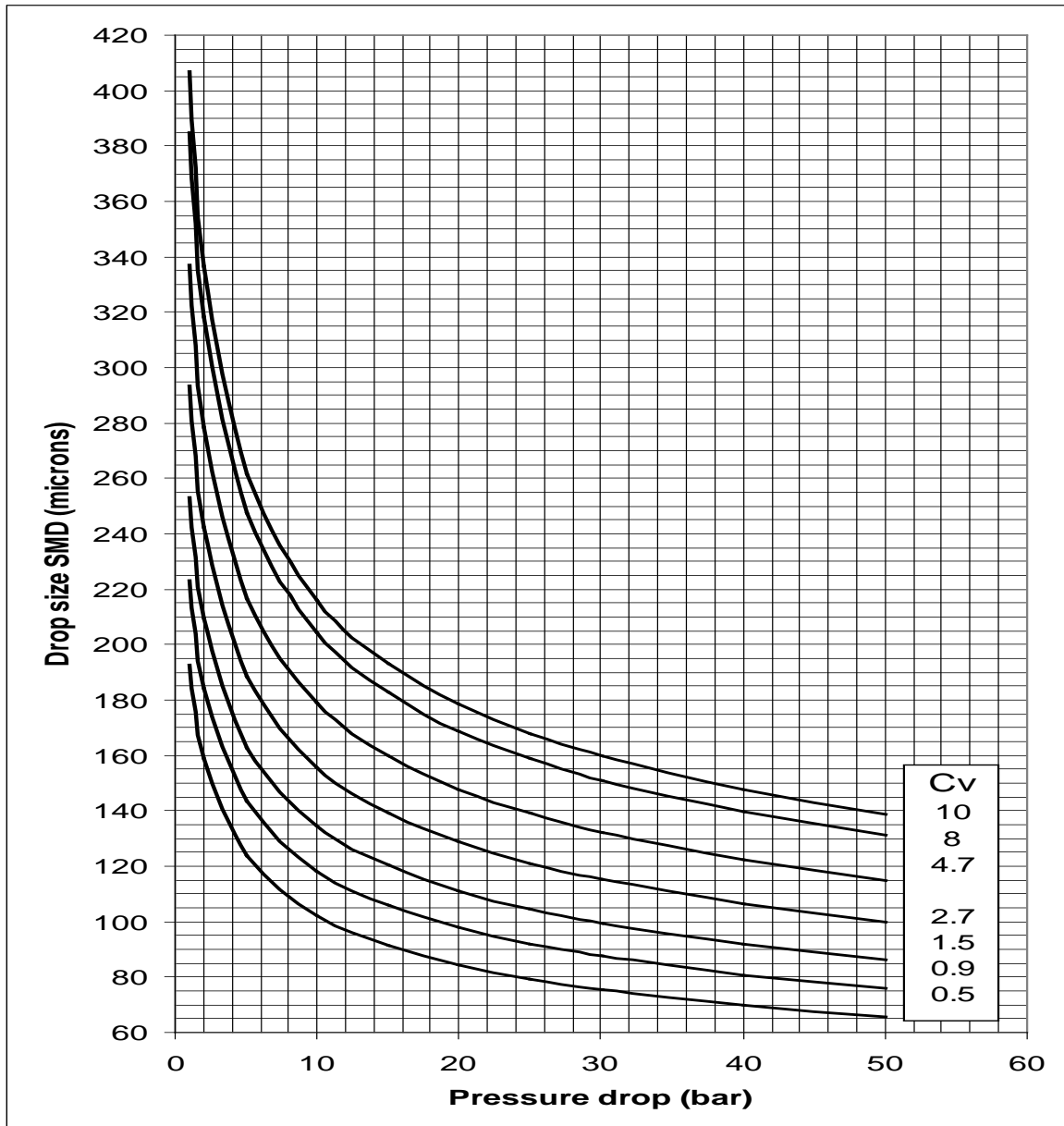
Figure D.1 Maximum Droplet Size Based on Cv and Pressure Drop
